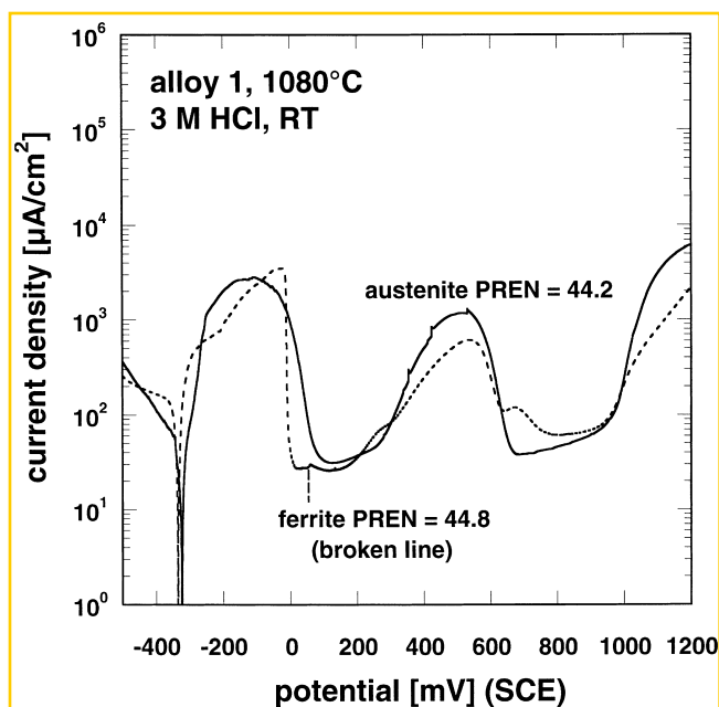
Fig. 8. Microelectrochemical polarisation curves of austenite and ferrite (in 3 M HCl at 23°C) of alloy 1 (solution annealed at 1080°, one step).
